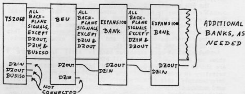
FIG 4. TS2068 WITH EXPANDED BUS AND DAISY CHAIN
